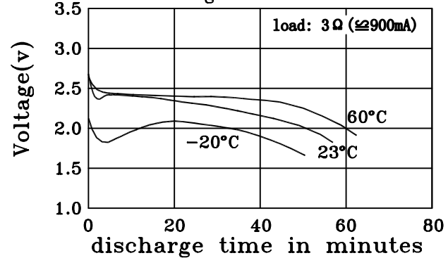
Discharge Characteristics
