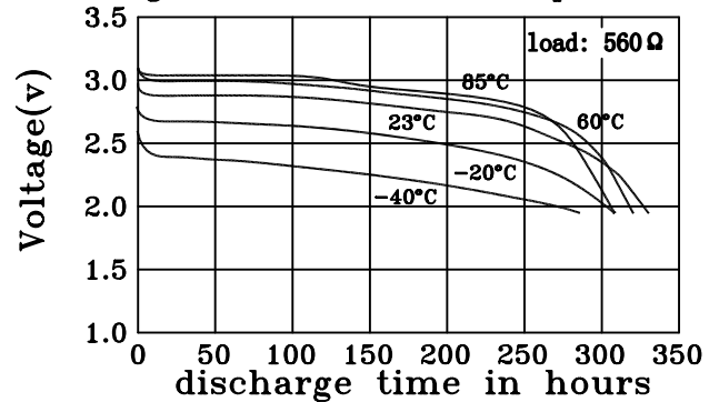
Discharge characteristics on temperature
